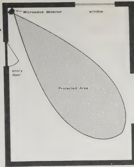
Typical microwave detector pattern (view from above).
